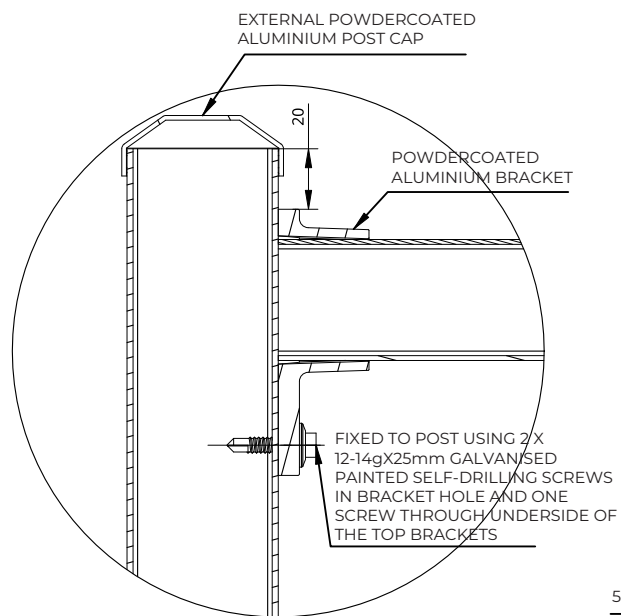
Detail A 1:2.5
